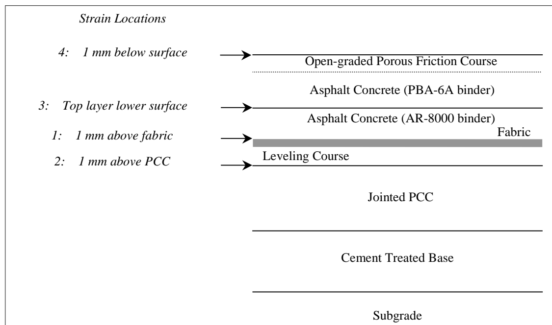
Figure 6. Pavement Representation Showing Locations at which Tensile and Shear Strains were Determined.
