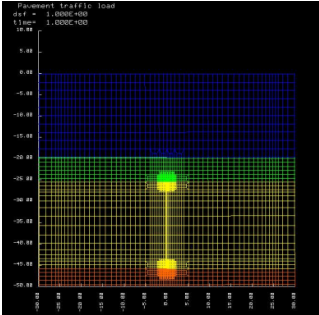
Figure 4. Finite Element Mesh used for Nike 2D Analyses; a Total of about 12,000 elements.
