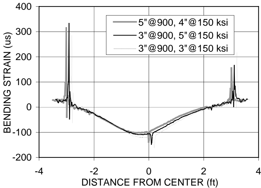
Figure 18. Comparison of Bending Strains in Mix just above PCC Joints/Cracks for Three Thicknesses Combinations of the PBA-6A and AR-8000 Mixes.
