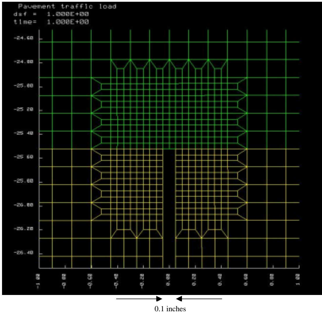
Figure 5. Close-up of Finite Element Mesh in the Vicinity of Crack.
