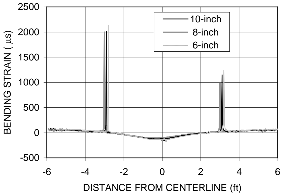
Figure 13. Effect of Layer Thickness on Strains in Mix just above Joints/Cracks in PCC.
