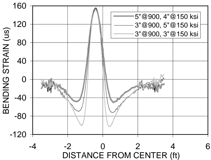
Figure 17. Comparison of Strains at Underside of Mix Just Above the Fabric Interlayer for Three Thickness Combinations of the PBA-6A and AR-8000 Mixes.
