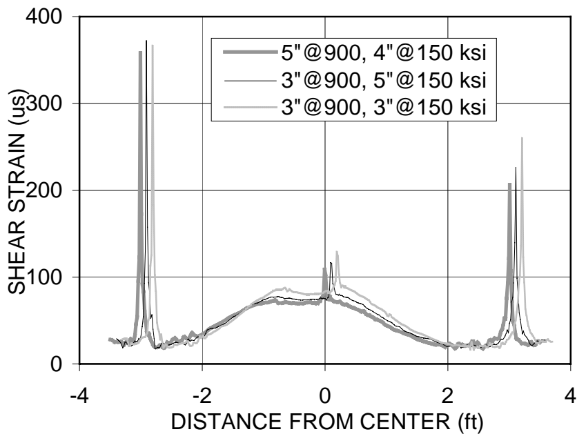
Figure 21. Comparison of Shear Strains in Mix just above Joints/Cracks in PCC Layer for Three Thickness Combinations of the PBA-6A and AR-8000 Mixes.
