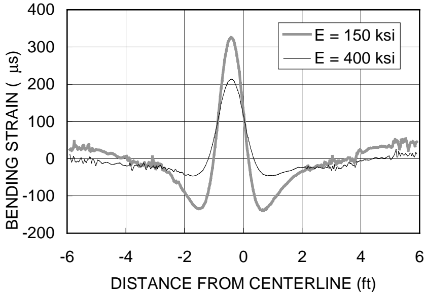
Figure 11. Influence of Overlay Stiffness on Strains in Layer Immediately Above Fabric Interlayer.
