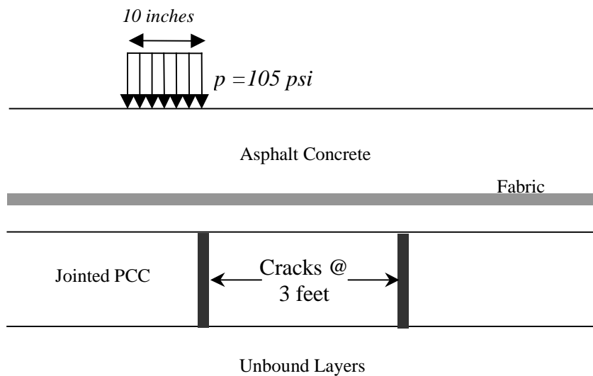
Figure 3. Pavement and Loading Configurations Used for Finite Element Analyses
