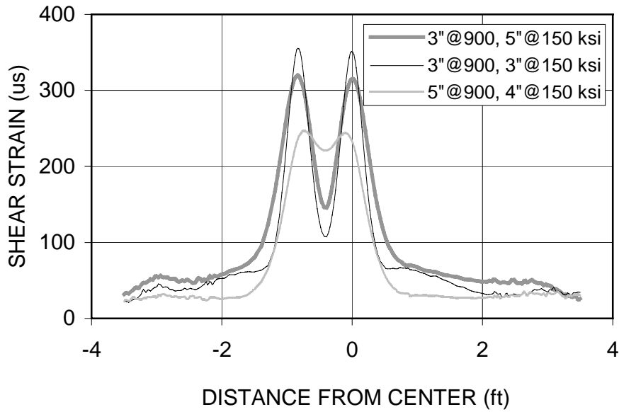
Figure 22. Comparison of Shear Strains near the Underside of the PBA-6A Mix for Three Thickness Combinations of the PBA-6A and AR-8000 Mixes.
