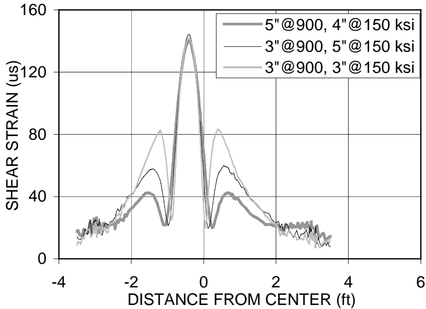
Figure 20. Comparison of Shear Strains in the Underside of the Mix Adjacent to the Fabric Interlayer for Three Thickness Combinations of PBA-6A and AR-8000 Mixes.
