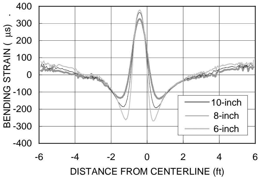
Figure 12. Effect of Surface Layer Thickness on Strains in Mix just above the Fabric Interlayer.
