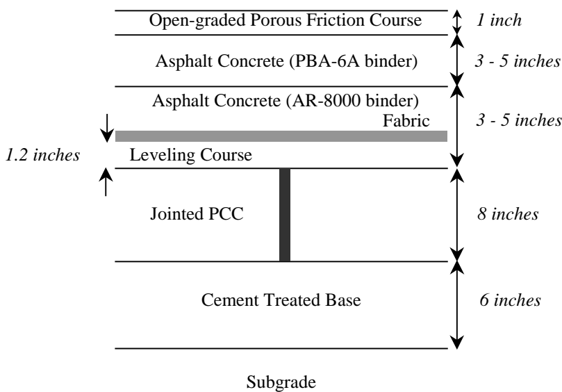
Figure 2 Pavement Systems Considered for Final Design
