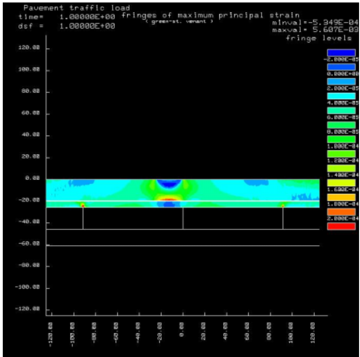
Figure 8. Fringes of Maximum Principal Strain in the Asphalt Concrete Layer for the Load Condition Shown in Figure 3.
