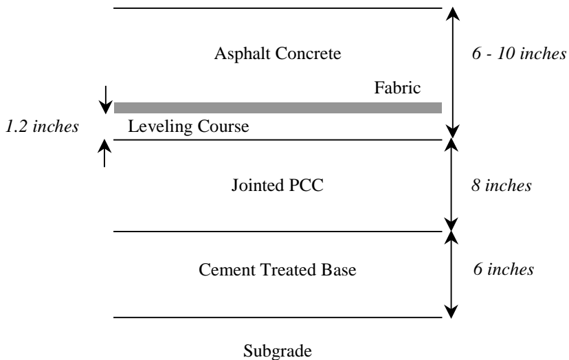
Figure 1 Pavement Representation for First Analysis Series
