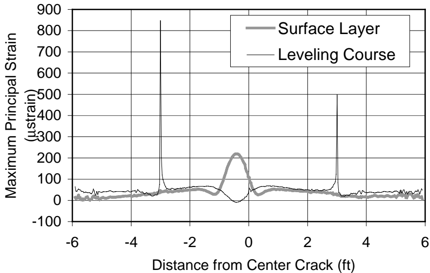
Figure 7. Tensile Strains Occurring in the Asphalt Concrete Layer in the Vicinity of Joints/Cracks Just Above (1mm) the Surface of the Concrete and Fabric Interlayer.
