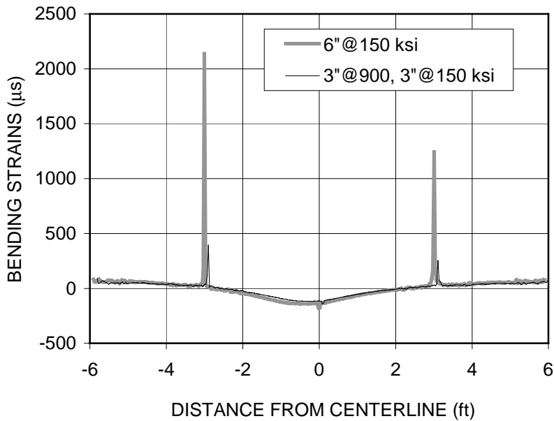
Figure 15. Comparison of Strains in Mix Just Above Joints/Cracks in PCC Layer for Single Layer (PBA-6A mix) and Composite Layer (PBA-6A mix and AR-8000 mix).
