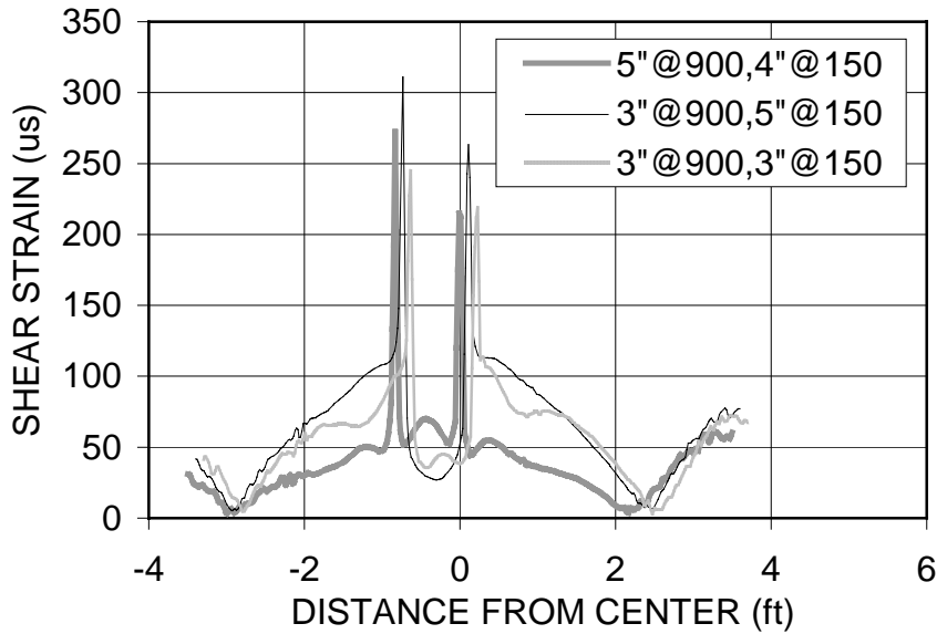
Figure 23. Comparison of Shear Strains near the Surface of PBA-6A Mix for Three Combinations of PBA-6A and AR-8000 Mixes.
