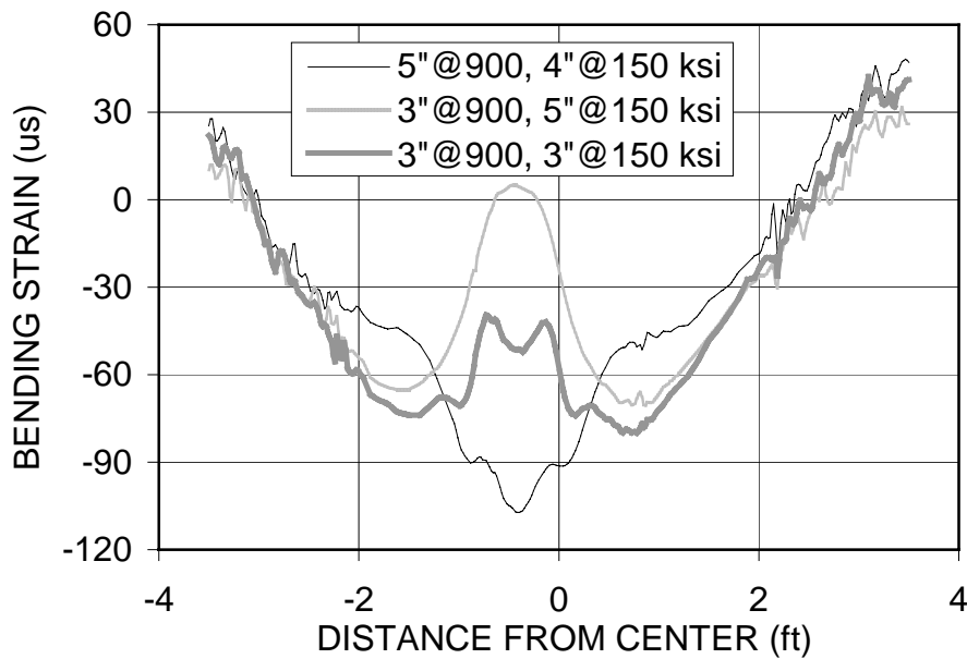
Figure 19. Comparison of Bending Strains in Bottom of Top Layer for Three Thickness Combinations of the PBA-6A and AR-8000 Mixes.
