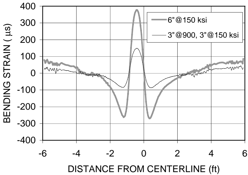
Figure 14. Comparison of Strains in Mix Immediately Above Fabric Layer for Single Layer (PBA-6A mix) and Composite Layer (PBA-6A mix and AR-8000 mix).
