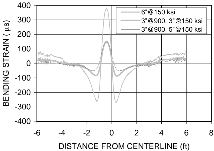
Figure 16. Comparison of Strains at Underside of the Mix just above the Fabric Interlayer for a PBA-6A Mix and Two Thickness Combinations of the PBA-6A and AR-8000 Mixes.
